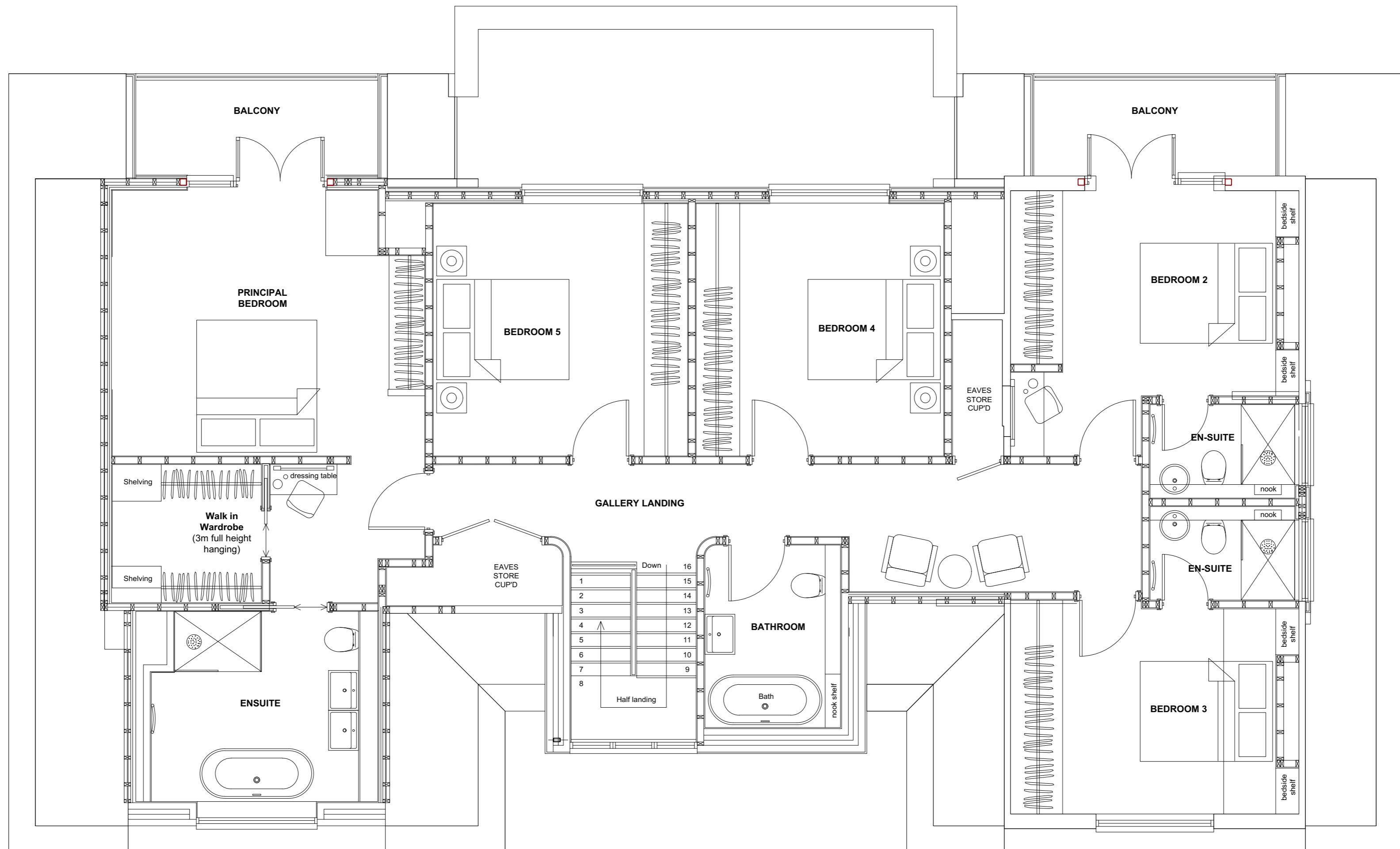
Proposed First Floor Plan Scale 1:50 @ A2
